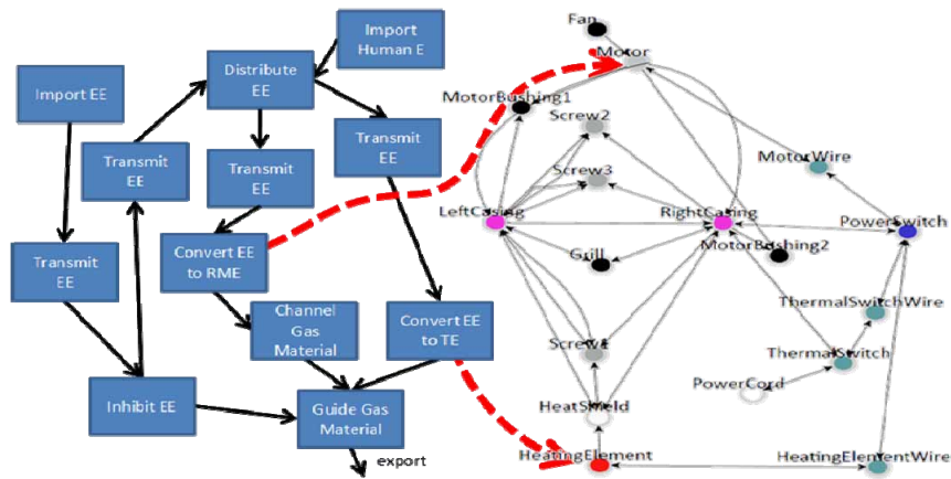
Figure 1. A function structure and a component flow graph (CFG) for a simple hair dryer. Arcs in both graphs include labels on the type of energy material or signal flow between the elements
